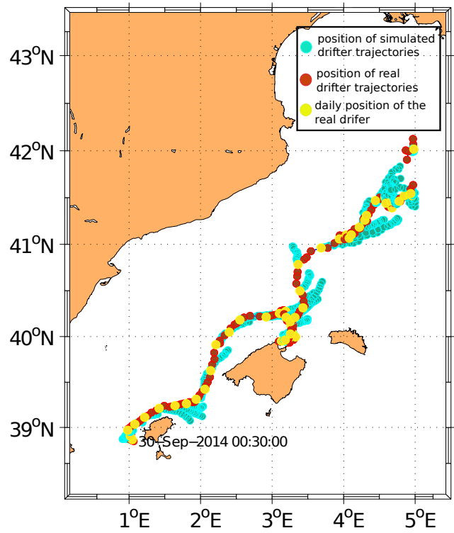
a) Comparison of virtual trajectories of particles advected with the IBI model velocity field with a real CODE drifter trajectory
