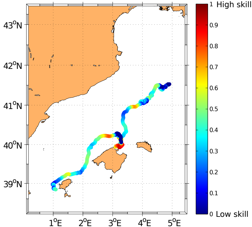
b) Model skill score after 72 hours of trajectory simulations
